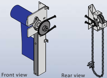
PULL CHAIN OPERATOR THROUGH WALL MOUNTING
